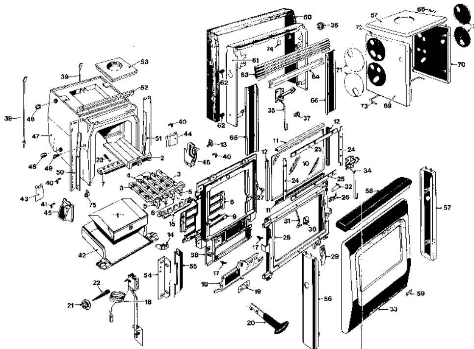
111 CONSORT, CAPRICE AND FREESTANDING CONSORT MODELS
